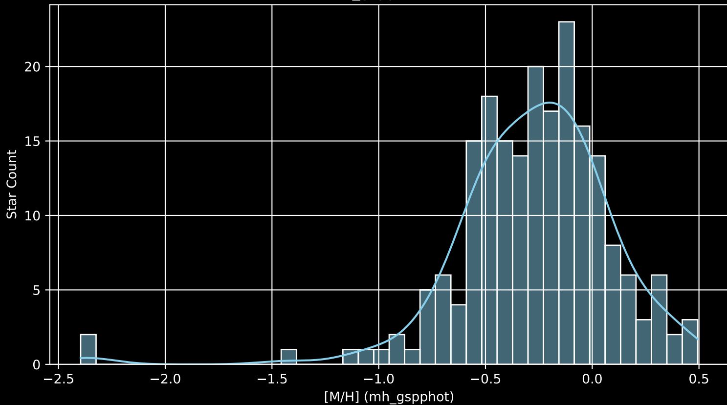
APOGEE DR17 Field: [130-60 [M/H] (mh_gspphot) (n= 204)
