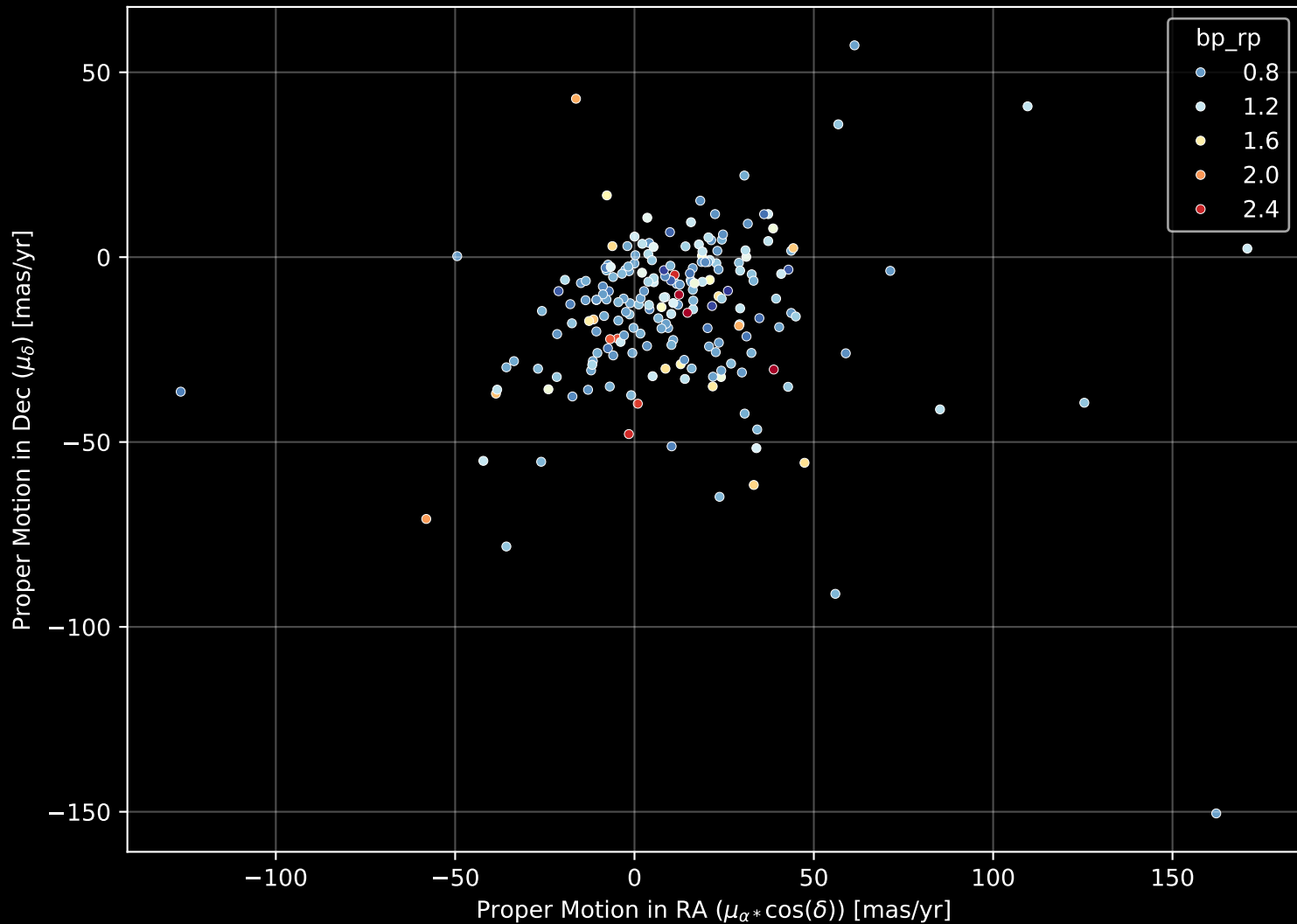
APOGEE DR17 Field: [130-60] Proper Motion Diagram (n= 204)
