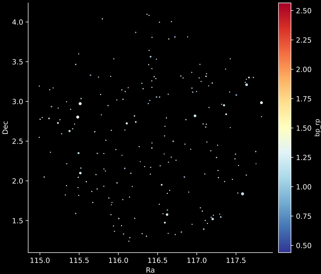
APOGEE DR17 Field: [130-60] Stars: 204
