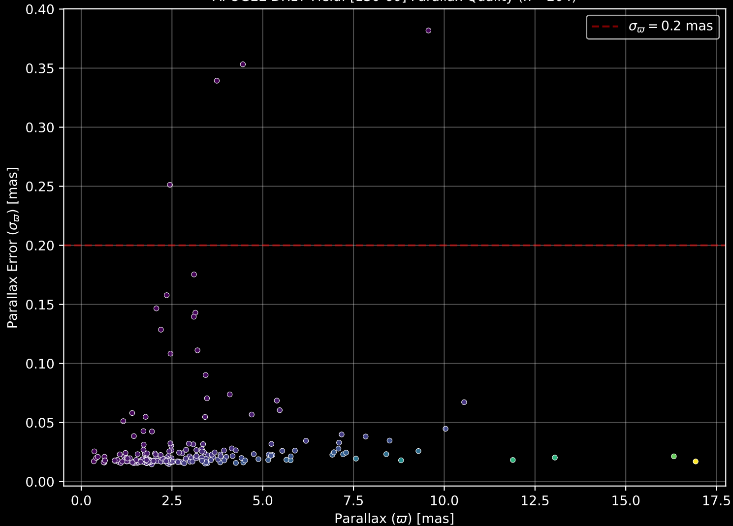
APOGEE DR17 Field: [130-60] Parallax Quality (n= 204)
