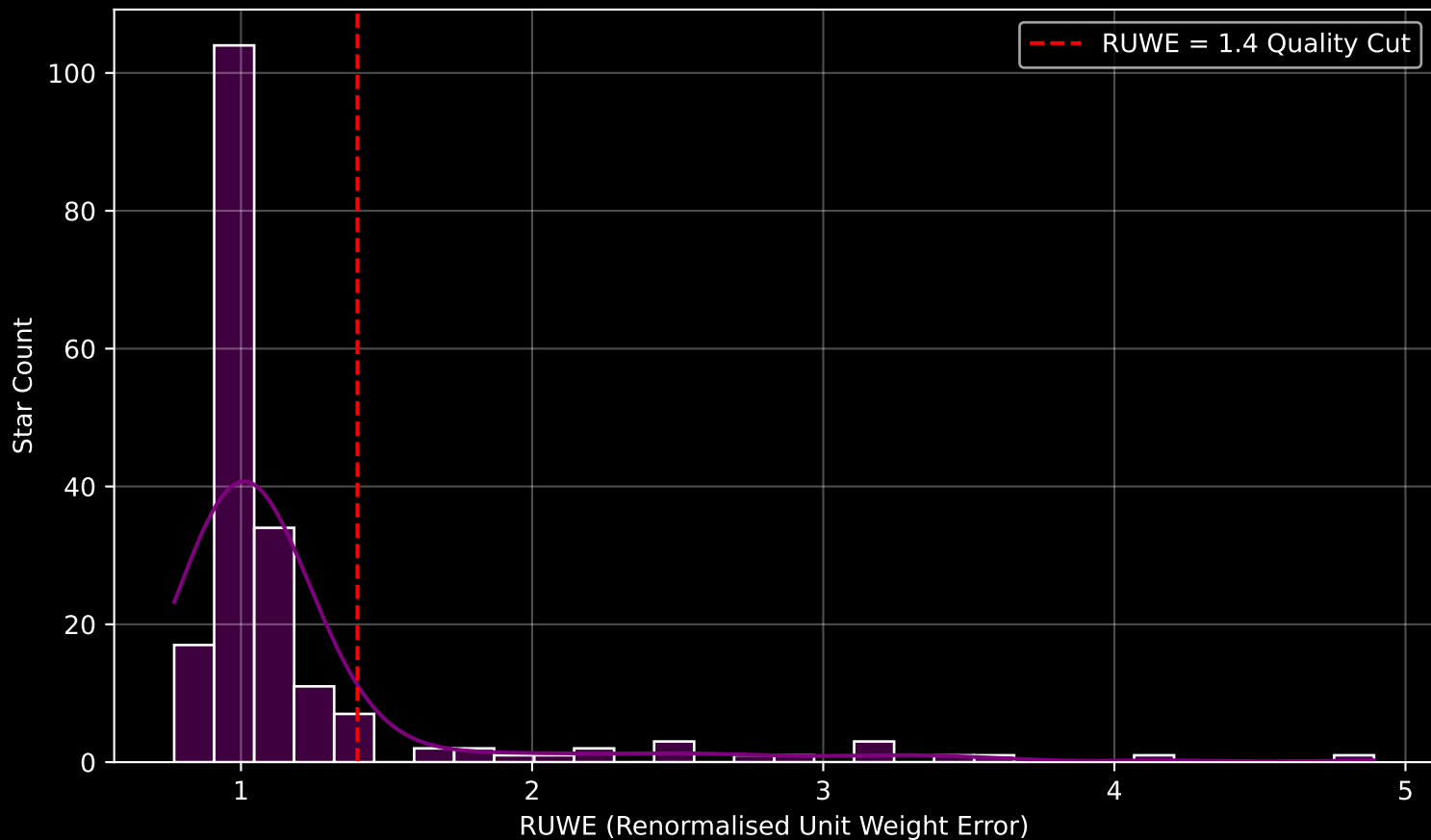
GAPOGEE DR17 Field [130-60] RUWE Distribution (n= 193)
